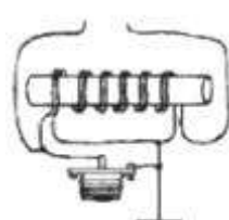
BALUN (HF)
